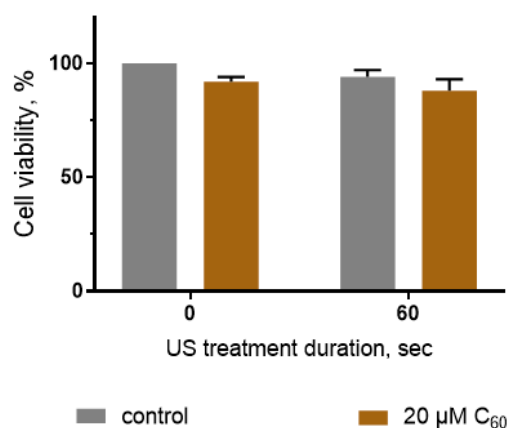
Figure 5. Viability of HEL 299 cells, incubated in the presence of 20 μM C 60 and treated with 1 MHz ultrasound (US).
