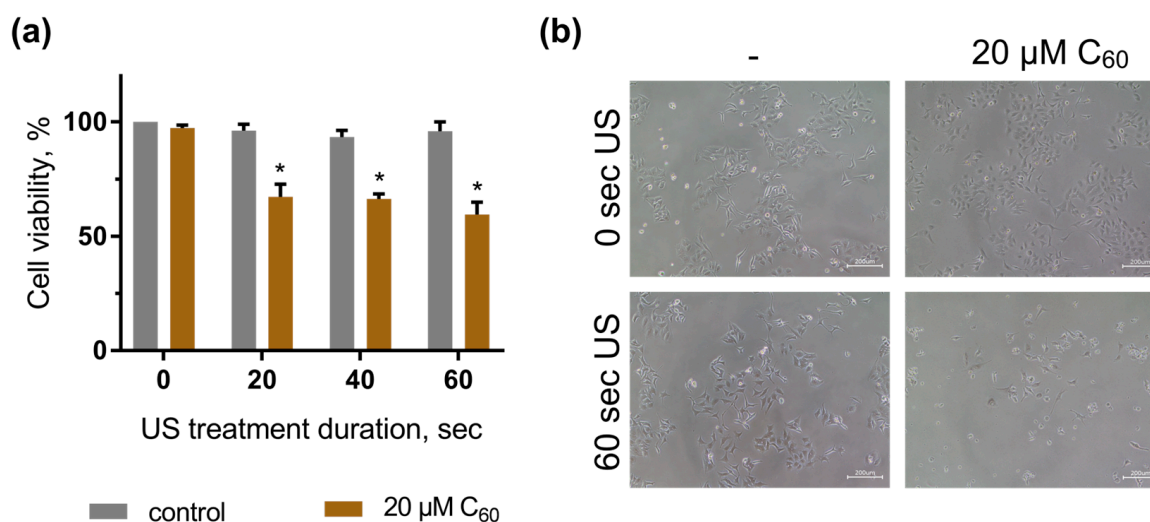
Figure 4. Viability of HeLa cells, incubated in the presence of 20 μM C 60 and treated with 1 MHz ultrasound (US): (a)—MTT assay, *— p \leq 0.01 in comparison with the viability of cells, treated with the respective duration of US; (b)—Phase contrast microscopy images of HeLa cells, incubated in the presence of 20 μM C 60 and treated with 60-s ultrasound, scale bar 200 μm.
