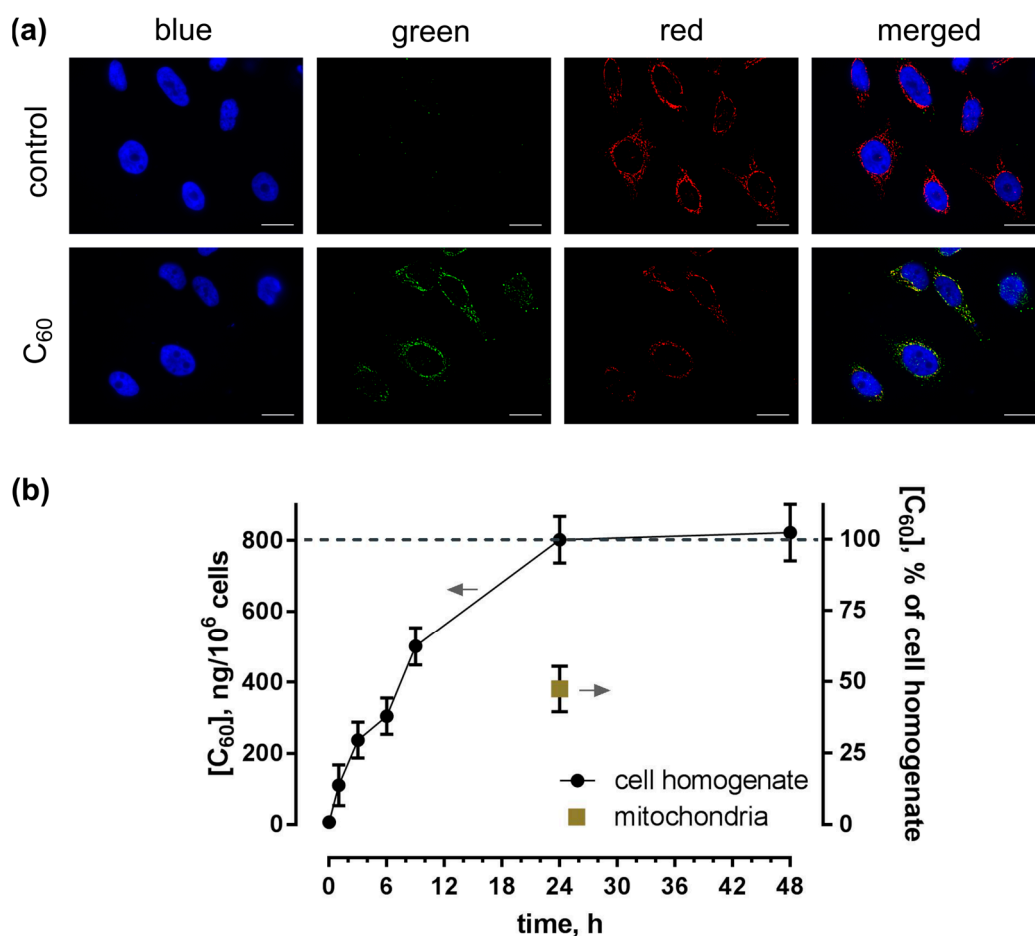
Figure 3. Uptake of C 60 in HeLa cells: (a)—Fluorescence microscopy images of HeLa cells, incubated for 24 h with 20 μM C 60 and stained with DAPI (blue), MitoTracker (red) and FITC-labeled antibody against C 60 (green), scale bar 20 μm; (b)—HPLC-ESI-MS analysis of C 60 content in toluene extracts from cell homogenate and mitochondrial fraction after incubation of cells with 20 μM C 60 .
