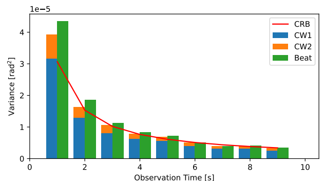
FIGURE 2. Cramér-Rao bound compared to simulation result for different observation times.
