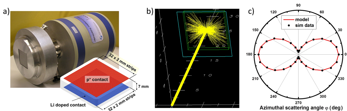
Figure 1. a) Photograph of the 2D Si(Li) polarimeter and a sketch of the crystal segmentation. b) Monte Carlo simulation of 100% linearly polarized 100 keV photons undergoing Compton scattering inside the detector crystal. c) Azimuthal scattering distribution of the reconstructed Compton events inside the detector. The red line shows an adjustment of the theoretical scattering distribution with the degree of linear polarization as a free parameter.
