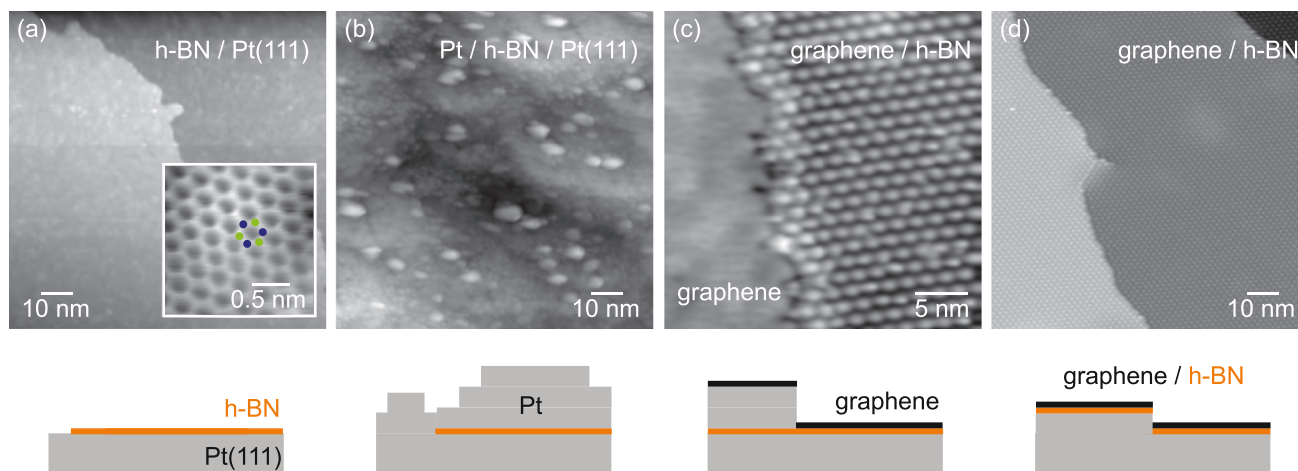
Figure 1. Preparation of graphene on h-BN. a) STM image of a single h-BN layer on Pt(111) (bias voltage: 2.4 V, tunneling current: 100 pA, size: 100 nm × 100 nm). Inset: Atomically resolved h-BN lattice with indicated positions of B and N (10 mV, 600 nA, 2 nm × 2 nm). b) STM image of h-BN-covered Pt(111) after deposition of a Pt film (1.15 V, 100 pA, 100 nm × 100 nm). Compact protrusions are due to Pt clusters residing on the closed metal film. c) STM image of a surface region where the graphene-covered Pt film (left) is juxtaposed to the graphene-h-BN stacking (right) by a Pt film step edge (0.5 V, 100 pA, 30 nm × 30 nm). d) STM data for the graphene-h-BN stacking on Pt(111) (1 V, 100 pA, 100 nm × 100 nm). The sketches under the STM images in (a-d) represent side views of the suggested stackings.
