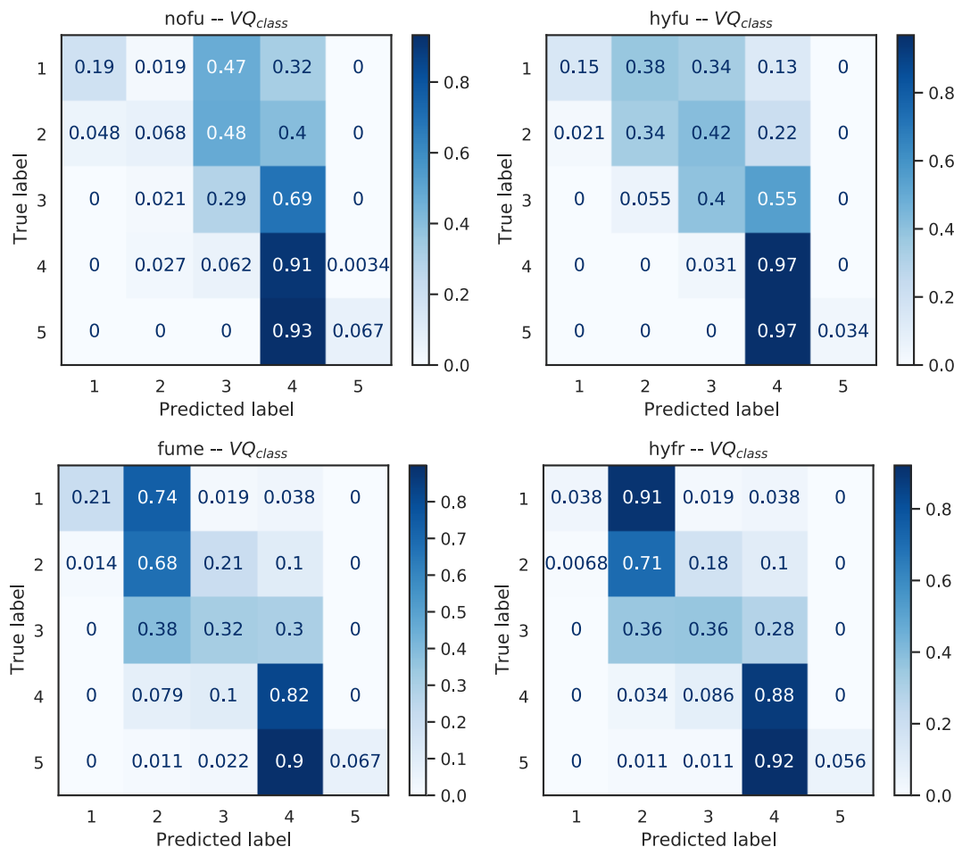
FIGURE 7. Confusion matrices for all models for VQ_{class} .
