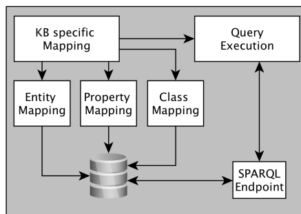
Fig. 3: Components specific for the Underlying Knowledge Base
