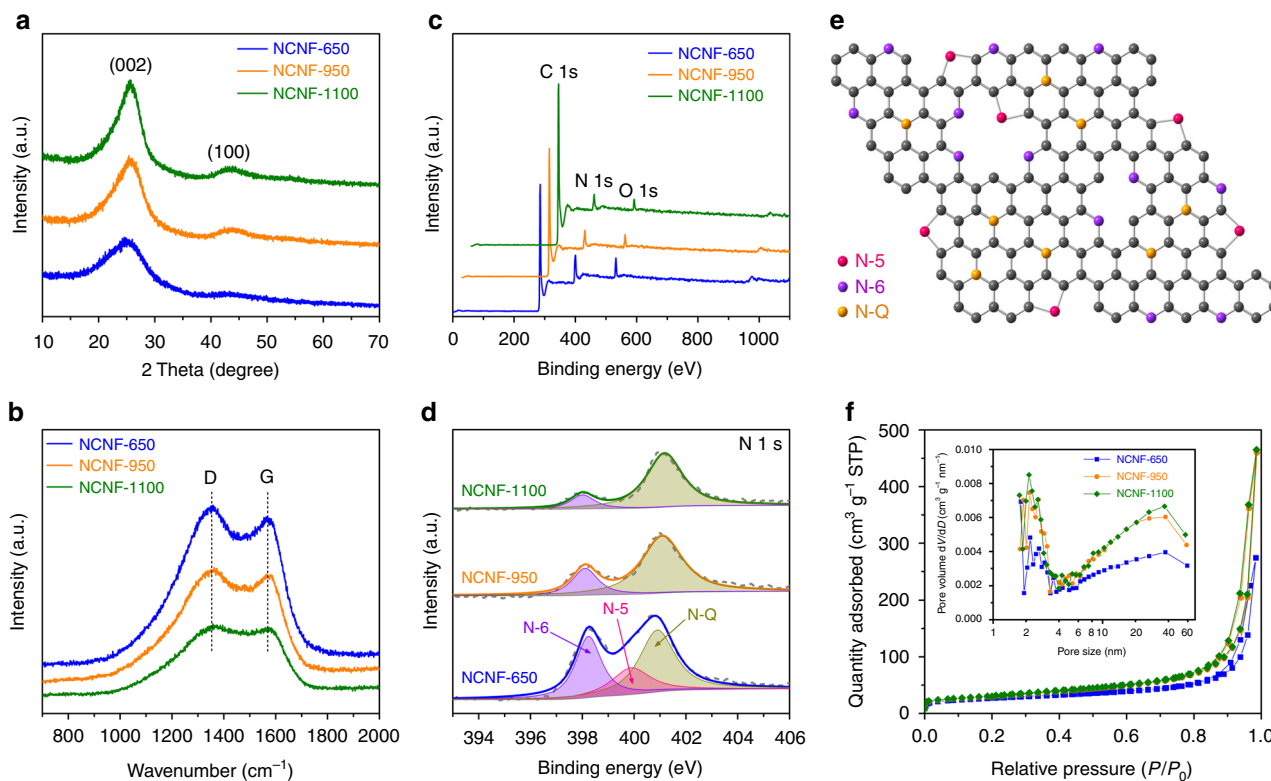
Fig. 2 Structure characterizations of NCNFs by spectroscopies. a XRD patterns. b Raman spectra. c XPS survey spectra. d N 1s core level XPS high-resolution spectra. e A schematic illustrating the structure of the N-doping species. f Nitrogen adsorption-desorption isotherms (inset shows the related pore size distribution)
