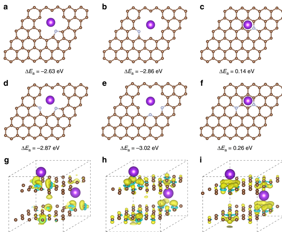
Fig. 6 Theoretical simulations of K-adsorption in different N-doped structures. Top view of a single K atom adsorbed in the N-5 ( a ), N-6 ( b ), and N-Q ( c ) structures and the corresponding adsorption energy. Top view of a single K atom adsorbed in the doped structures with two nitrogen atoms and the corresponding adsorption energy: d one N-5 and one N-6 atoms; e two N-6 atoms; f two N-Q atoms. Electron density differences of K adsorbed in the N-5 ( g ), N-6 ( h ), and N-Q ( i ) structures. Yellow and blue areas represent increased and decreased electron density, respectively. The isosurfaces are the 0.0015 electron bohr 3 . Brown, silver, and purple balls represent carbon, nitrogen, and potassium atoms, respectively
