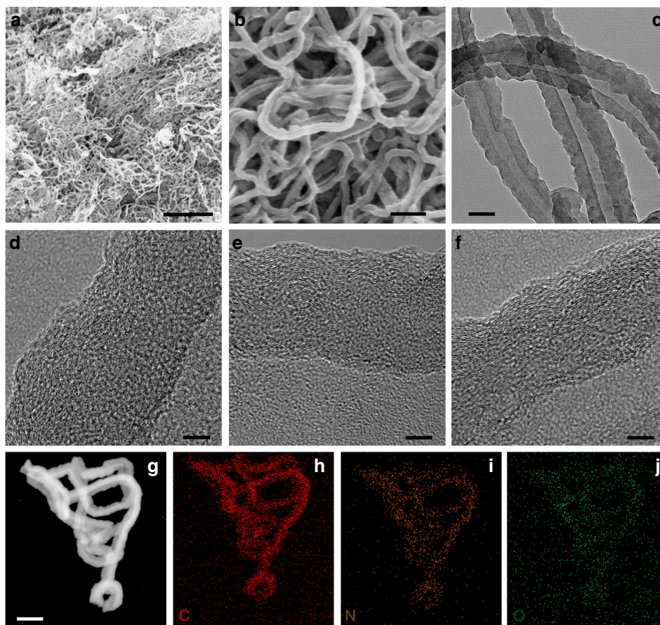
Fig. 1 Structure characterizations of NCNFs by electron microscopies. a, b SEM and c TEM images of NCNF-650. HRTEM images of NCNF-650 ( d ), NCNF-950 ( e ), and NCNF-1100 ( f ). g–j Images of element mapping of C, N, and O for NCNF-650. Scale bars: 2 \mu\text{m} ( a ); 200 nm ( b ); 50 nm ( c ); 5 nm ( d–f ); 100 nm ( g )
