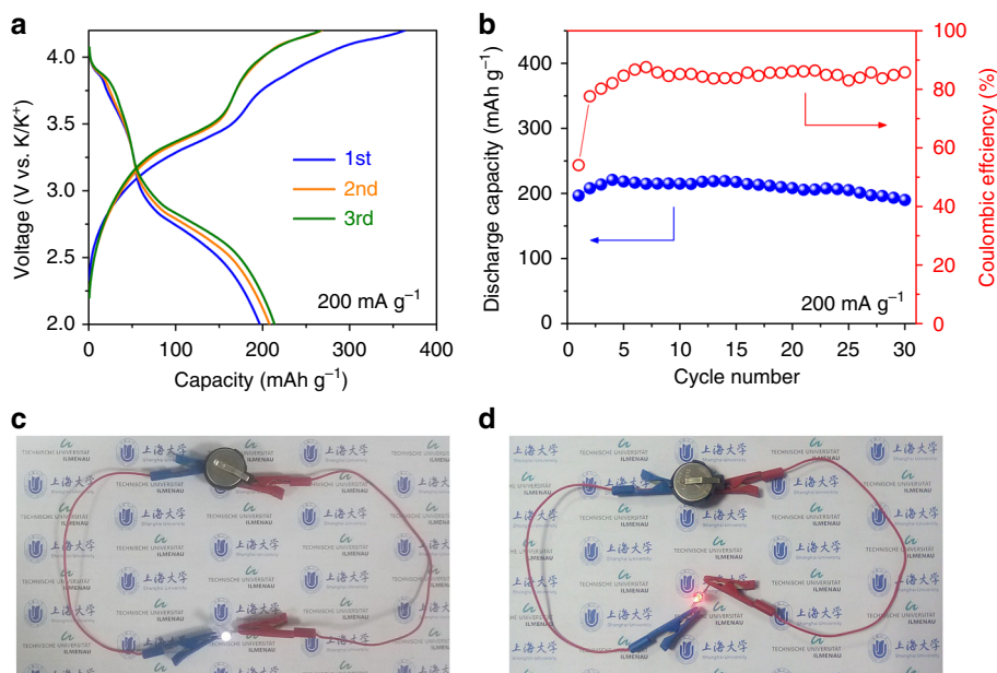
Fig. 5 Electrochemical performances of the NCNF-650/KPB full cell. Galvanostatic charge/discharge profiles ( a ) and cycling performance ( b ) at a current density of 200 \text{ mA g}^{-1} . Optical photographs of a white LED ( c ) and a red LED ( d ) lightened by the full cell
