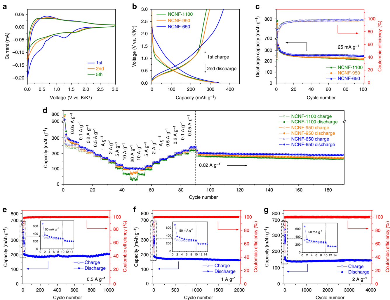
Fig. 3 Electrochemical performance of NCNFs as PIB anodes in half cells. a CV curves of NCNF-650. b First charge and second discharge profiles of NCNFs. c Cycling performance of NCNFs at a current density of 25 \text{ mA g}^{-1} . d Rate performance of NCNFs with rates ranging from 0.05 to 20 \text{ A g}^{-1} . Long-term cycling performance of NCNF-650 at high rates of 0.5 ( e ), 1 ( f ), and 2 \text{ A g}^{-1} ( g )
