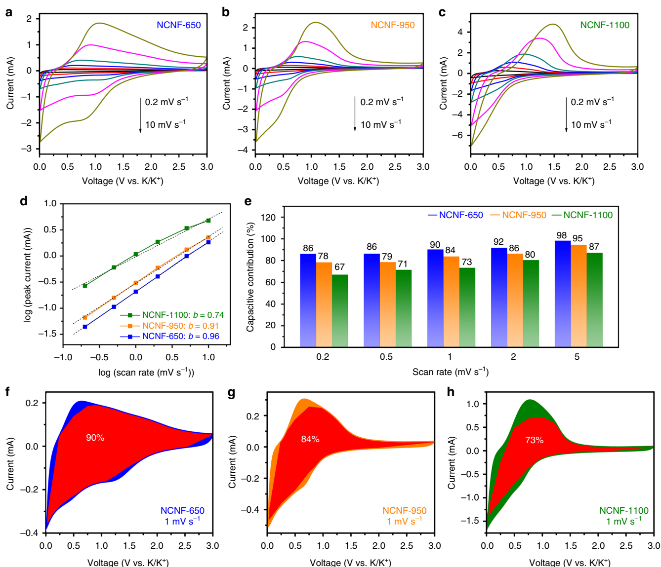
Fig. 4 Quantitative analysis of surface-dominated K-storage in NCNFs. CV curves of NCNF-650 ( a ), NCNF-950 ( b ), and NCNF-1100 ( c ) at various scan rates of 0.2 to 10 \text{mV s}^{-1} . d b value determination. e Contribution of the surface process in the NCNFs at different scan rates. Contribution of the surface process at scan rate of 1 \text{mV s}^{-1} in NCNF-650 ( f ), NCNF-950 ( g ), and NCNF-1100 ( h )
