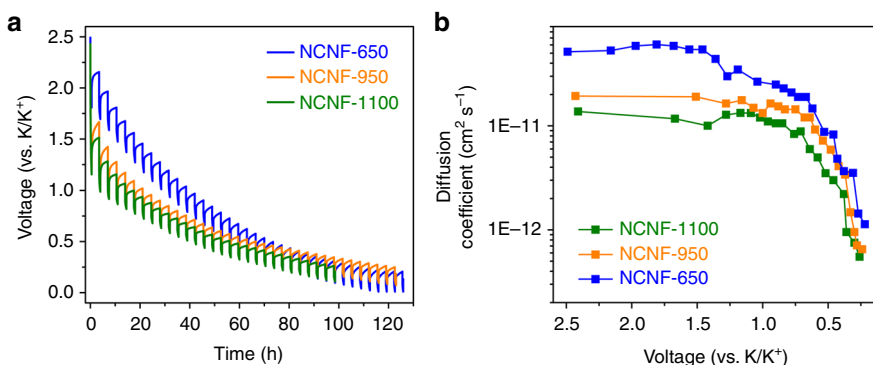
Fig. 7 Study of the K-ion diffusion coefficient of the NCNF electrodes. a GITT profiles of the discharging process. b The K-ion diffusion coefficient as a function of the state of discharging process
