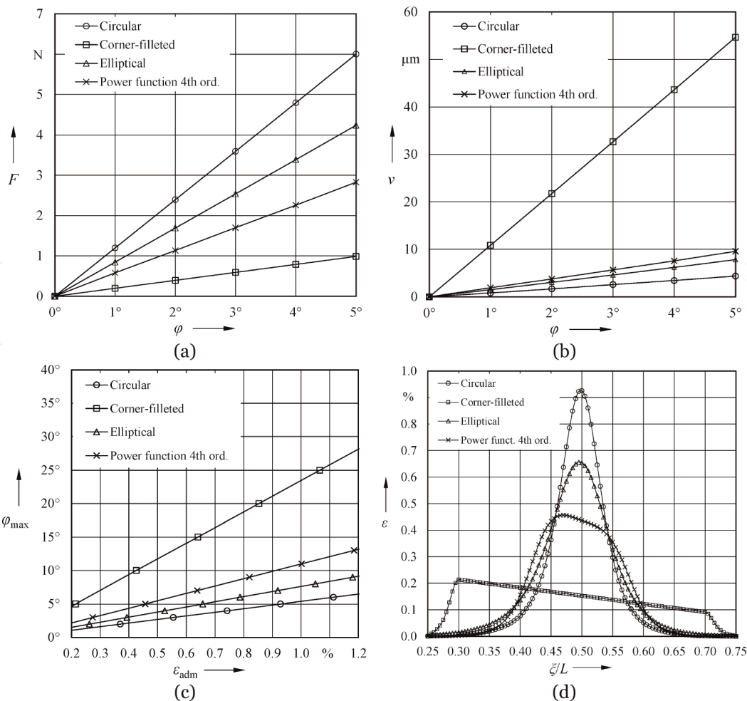
Figure 9. Analytical results for the influence of the flexure hinge contour on the hinge properties ( \beta_L = 2 , \beta_l = 1 , \beta_h = 0.03 , \beta_w = 0.6 , force load): (a) bending stiffness, (b) axis shift, (c) maximum angular deflection, and (d) outer fiber strain distribution for \varphi = 5^\circ .
