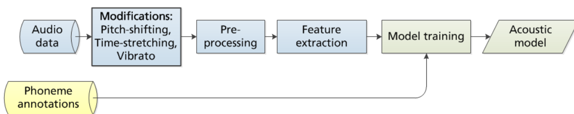
Figure 5.5: Overview of the “songified” phoneme recognition training process.
