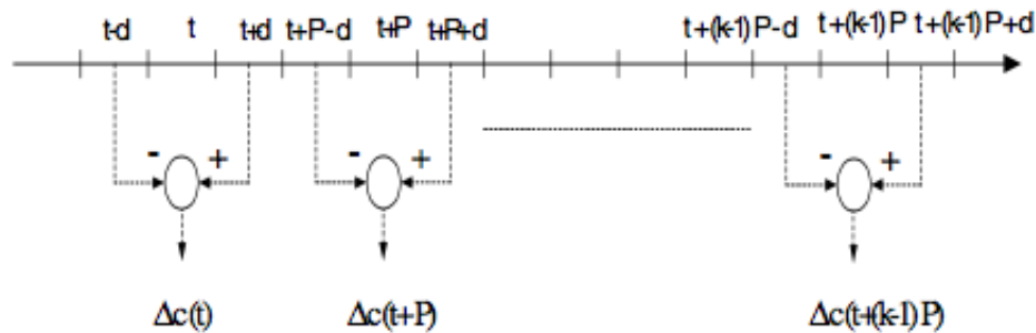
Figure 2.4: The SDC calculation at frame t . [14]
