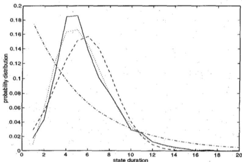
Figure 7.6: An example of the empiric duration distribution of one phoneme state (solid line) and three approximations: Gaussian (dashed), geometric(dash-dot), and gamma (dotted). [189]
