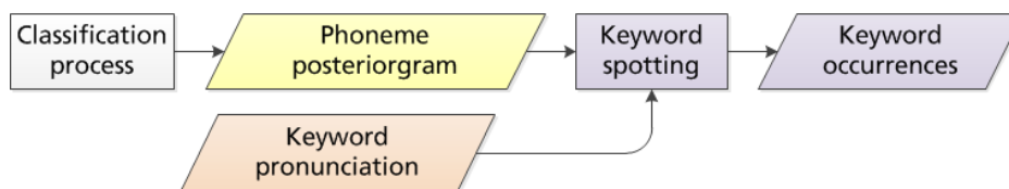
Figure 7.2: Schematic of the procedure for keyword spotting.
