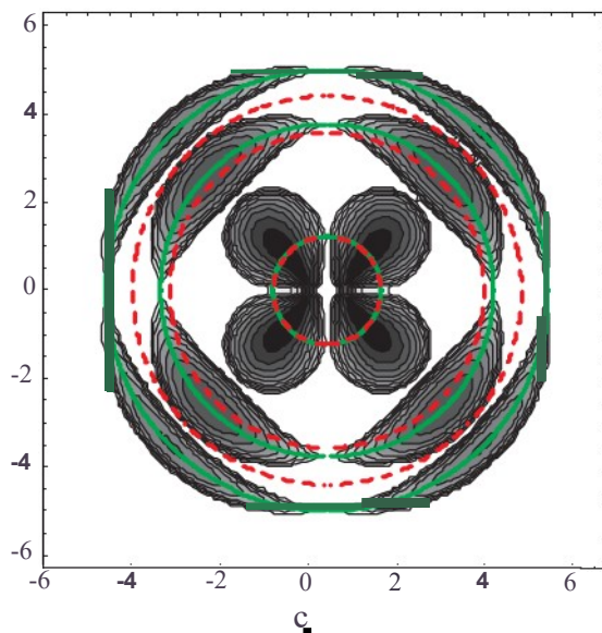
Figure 5.22: Growth rate obtained by solving Eq. 3.16 with 1 keV temperature, 7 \times 10^{16} \text{ W/cm}^2 perpendicular incidence and ne/nc = 0.24 plasma density for the innermost, 0.17 for the middle and 0.1 for the outermost curve. The red dashed circles are the TPD circles calculated using Eq. 3.33 and the green solid circles are the exact TPD circles.
