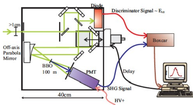
Figure 6.9: Multishot SHG autocorrelator (AC) used in the measurements. Special properties are the large supported beam diameter, the discriminator diode, the high sensitivity due to the photomultiplier tube (PMT) and the large supported bandwidth due to the thin beam splitter and BBO and to the focusing with off-axis parabola mirror.
