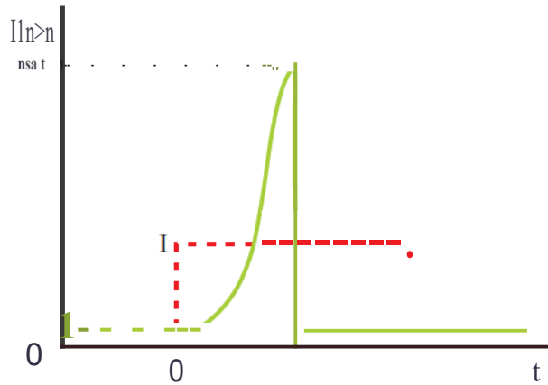
Figure 6.19: Suggested model of plasma wave saturation. The electron plasma wave amplitude ( nTPD ) and the laser intensity ( J ) as a function of time. The time t_s marks the point where saturation ( nsat ) is reached from the initial thermal noise ( nth ) and \tau is the pulse duration.
