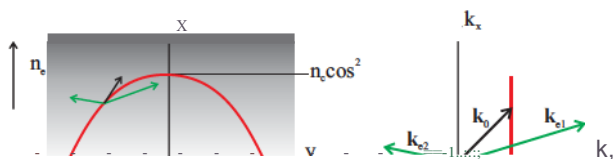
Figure 3.3: Propagation of the laser light in the plasma (red lines) and the TPD in the normal space and in the k space. The black arrow is the laser wavevector, and the green arrows correspond to the plasma waves.
