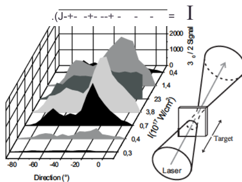
Figure 5.9: 3w_0/2 angular distributions with different intensities and a 50 ps prepulse. The small picture on the right depicts how the intensity was changed. Correspondingly the intensity axis has its maximum in the middle. The double-peaked structure disappears at the highest intensity.
