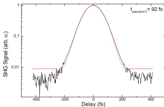
Figure 6.12: Test of the AC supported bandwidth using a Vitesse oscillator.
