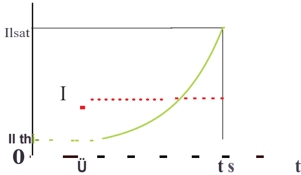
Figure 4.9: The electron plasma wave amplitude (nTPD) and the laser intensity ( I ) as a function of time. The time t_s marks the point where saturation (nsat) is reached from the initial thermal noise (11th) and \tau is the pulse duration.
