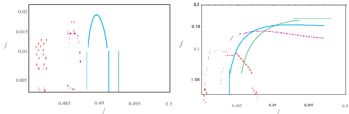
Figure 5.23: The TPD growth rate at an intensity of 2 \times 10^{16} \text{ W / cm}^2 (left) and 10^{18} \text{ W / cm}^2 (right), 1 keV temperature and an electron density of ne/nc = 0.1 red thick dashed line, 0.17 purple dashed-dotted thick line, 0.2 blue solid thick line and 0.245 green solid thin line.
