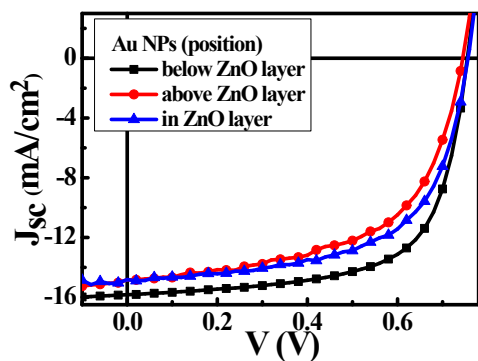
Fig. S4. Impact of Au NPs position on the device performance. The device with Au NPs at the interface of ITO/ZnO presents the best performance. The direct contact of Au NPs with ITO glass is helpful for collecting the charges in the device. When the Au NPs are inserted in the ZnO layer, the efficiency becomes lower. In this case, the charge collecting efficiency of the structure could not be improved. For the device with Au NPs on the top of ZnO layer, the direct exposure of the metallic nanoparticles to the polymer layer could cause the recombination of the photo-generated charge carriers, which deteriorates the device efficiency.
