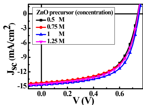
Fig. S2. The optimization of the device performance by the thicknesses of ZnO layer. The ZnO film prepared from the 1 M precursor solution has a thickness of 35 nm and the relevant device presents the best performance. The devices with ZnO film prepared from a lower concentrated precursor solution show a lower performance, probably due to the imperfect coverage of the ZnO thin film on the substrate. In addition, the performance decrease of the device with a thicker layer of ZnO could be attributed to the inefficient charge transport, due to the imperfect crystal quality of the ZnO film.
