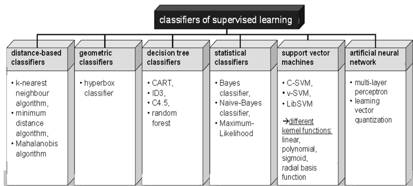
Figure 1. Classifiers of supervised learning [6].
