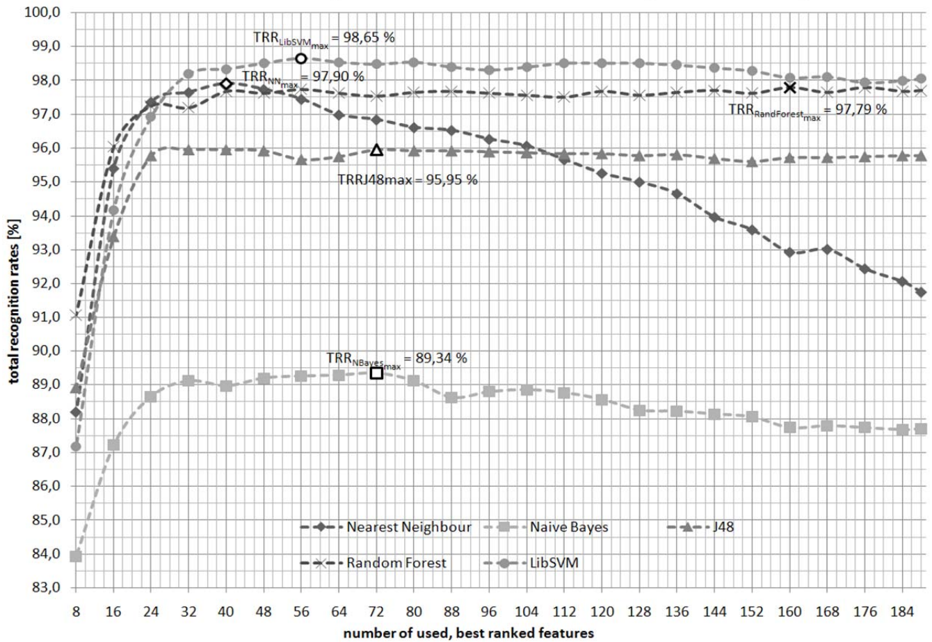
Figure 5. Classification performance of different classifiers versus dimensionality of the feature space by using the number of best ranked features.
