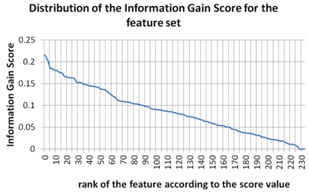
Figure 10. Feature scoring.
