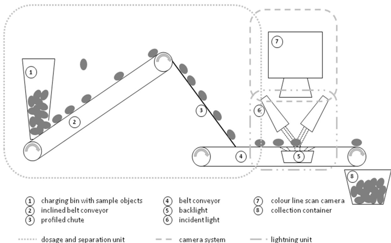
Figure 7. Hardware setup for image acquisition of mineral aggregates.
