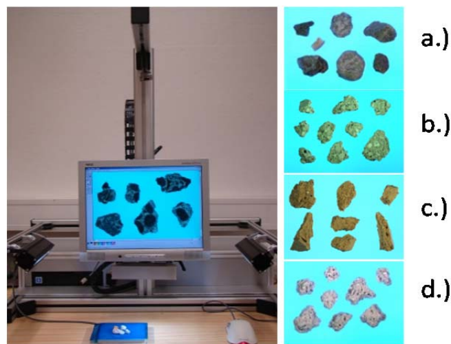
Figure 3. Image system "QI Inspector" [19] and images of samples a) concrete, b) lightweight concrete, c) brick and d) aerated concrete.
