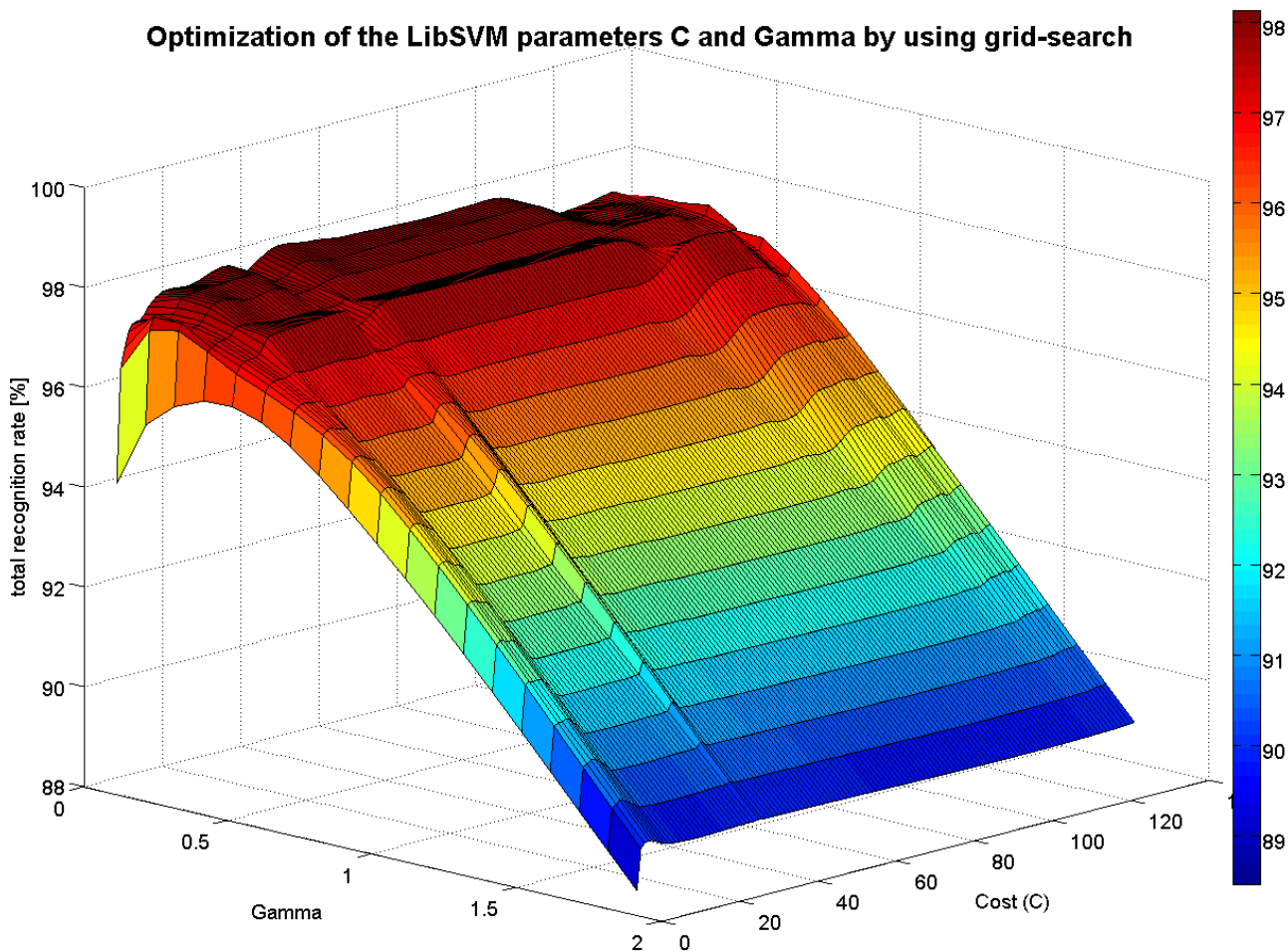
Figure 4. Surface plot of parameter optimization of LibSVM.
