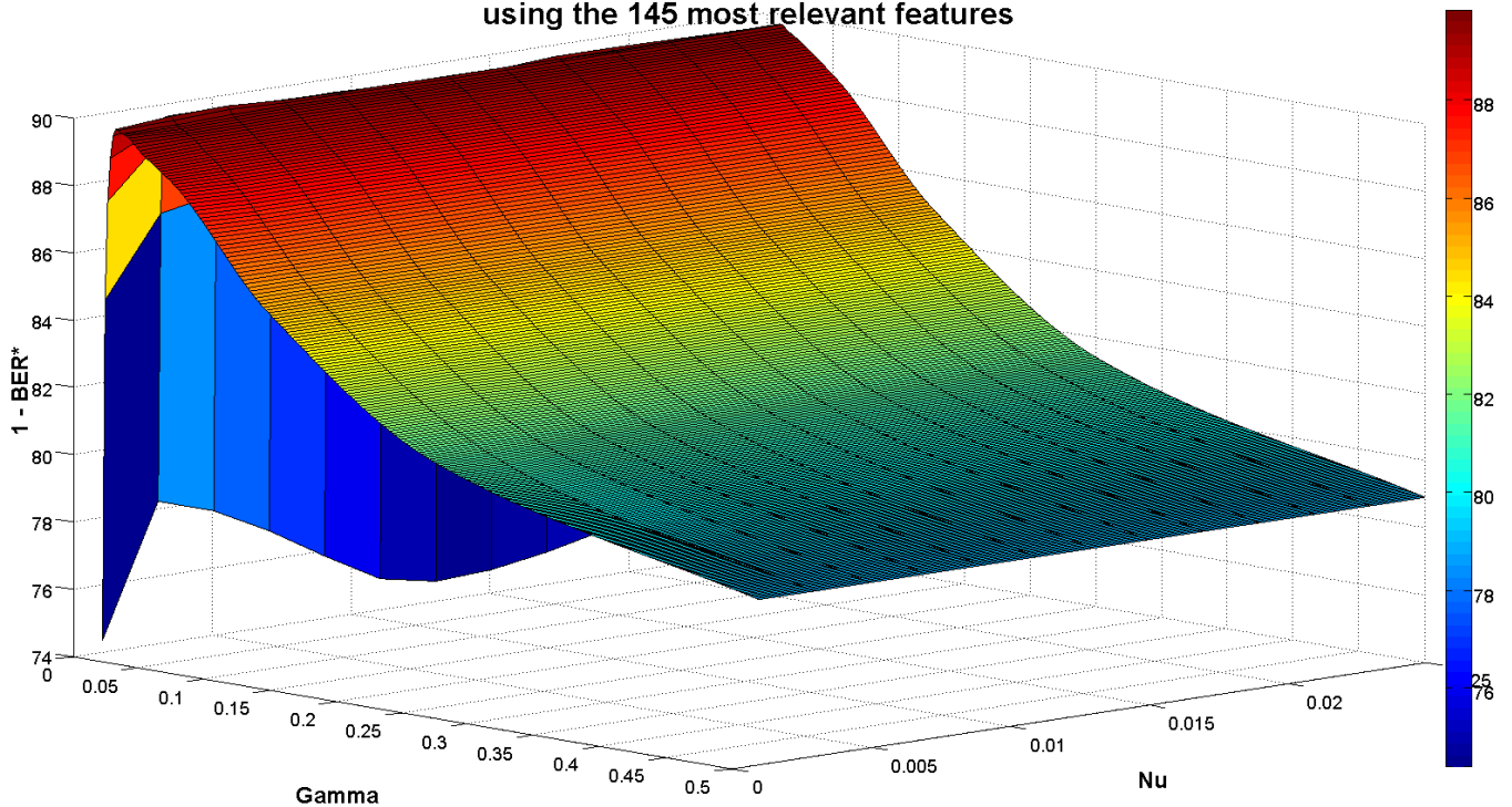
Figure 12 Results from the grid search algorithm.
