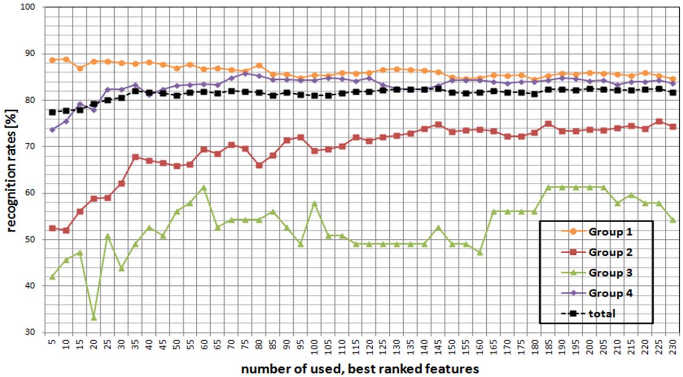
Figure 11. Filter-based feature selection.
