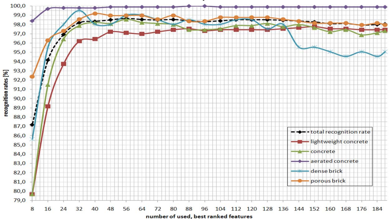
Figure 6. SVM performance versus dimensionality of the feature space by using the number of best ranked features.
