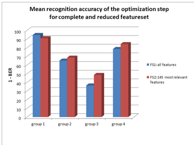
Figure 15. Mean accuracy of different parameter combinations during the optimization for FS1 and FS2.
