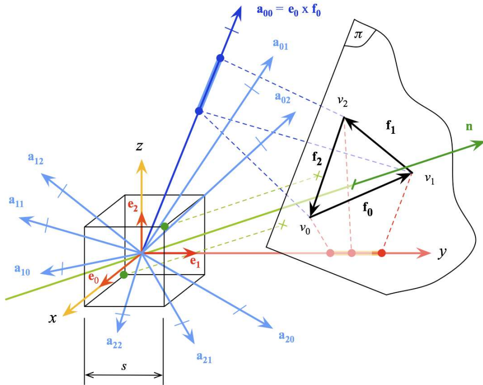
Figure 3: Collision detection between triangle and voxel using the Separating Axis Theorem (SAT). Red: three coordinate axes \{\mathbf{e}_0, \mathbf{e}_1, \mathbf{e}_2\} ; Green: the normal axis \mathbf{n} ; Blue: nine cross-axes \{\mathbf{a}_{ij}\} .
