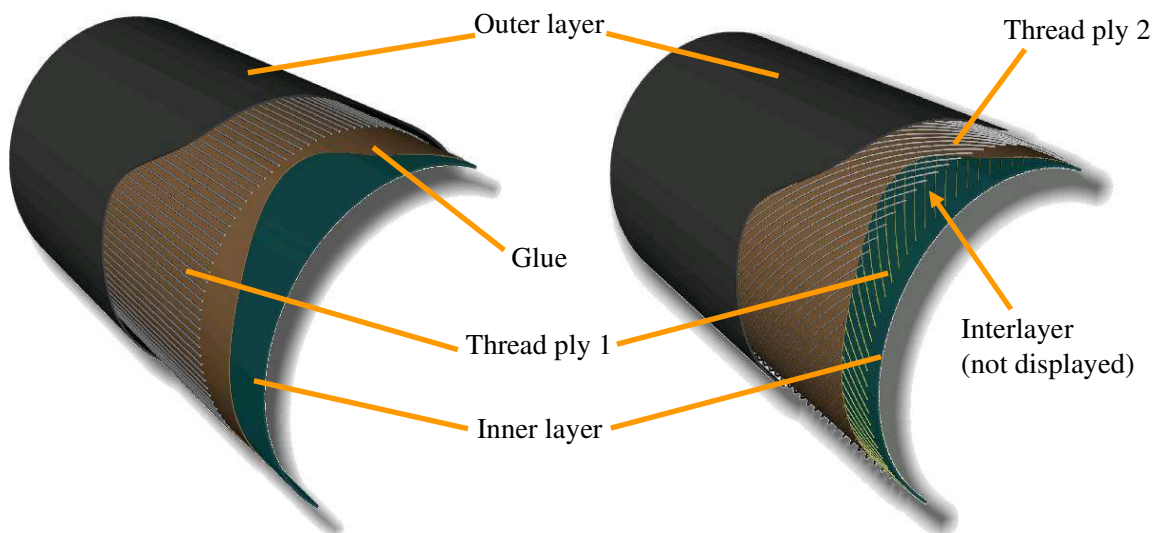
Figure 3: Design of axial bellow (left) and cross ply bellow (right) [2]
