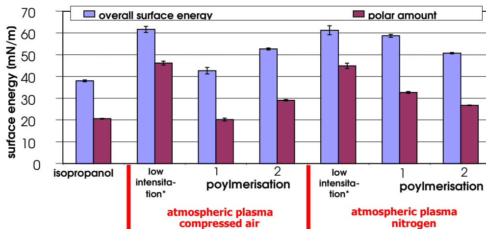
Figure 2: Results of the contact angle measurement on float glass after plasma activation and plasma polymerisation with compressed air and nitrogen
