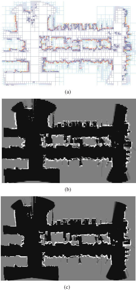
Fig. 4. (a) Leaf nodes of an N^d -tree map with N = 2, d = 2 (b) Same N^d -tree map where the leaf nodes are colored according to their occupancy value. (white=1, black=0) (c) Grid map with a fixed resolution of 0.1 m
