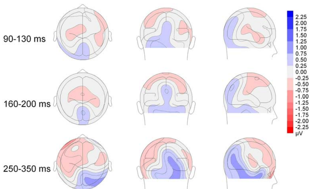
Figure 10: Voltage maps (spherical spline interpolation, 110^\circ equidistant projection) for the ERP difference (left-minus right-adaptation) averaged across test stimulus. Note the right posterior positivity (in blue) \sim 250-350 ms and the absence of direction-specific adaptation effects in the preceding P100 and N170 time segments.
